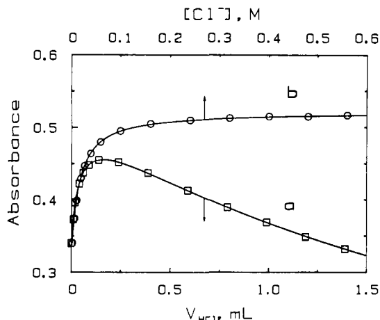
Figure 1. (a) Absorbance change in the spectrophotometric titration of \text{ICl}_2^- with 1.00 M HCl ( V_{\text{HCl}} ). Conditions: 2.50 mL of 1.90 \times 10^{-3} M [\text{ICl}_2^-]_{\text{init}} in 1.00 M \text{HClO}_4 at 25.0 °C, 1.00-cm cell, 343 nm. (b) Absorbance versus the iteratively calculated chloride concentration.
