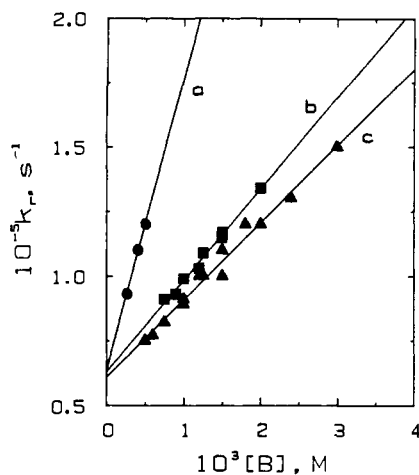
Figure 4. Rate constants from PAF measurements of the hydrolysis of \text{ICl}_2^- as a function of base concentrations. [\text{Cl}^-] = 0.50 \text{ M} , 230 nm. Key: (a) [\text{B}] = [\text{OH}^-] , [\text{ICl}_2^-]_{\text{init}} = 1.1 \times 10^{-5} \text{ M} ; (b) [\text{B}] = [\text{CO}_3]_{\text{T}} , \text{p}[\text{H}^+] = 9.2\text{--}9.7 ; (c) [\text{B}] = [\text{PO}_4]_{\text{T}} , \text{p}[\text{H}^+] = 6.1\text{--}7.1 . [\text{ICl}_2^-]_{\text{init}} = 3.0 \times 10^{-5} \text{ M} for (b) and (c).
