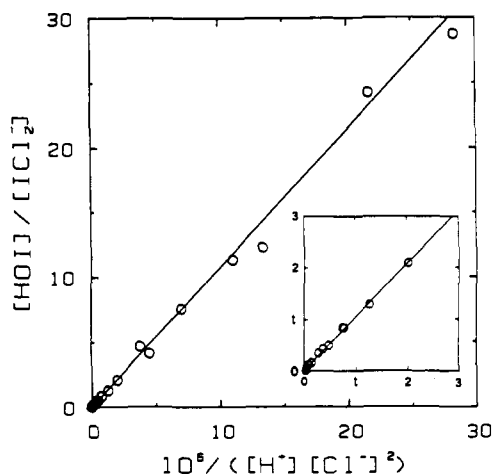
Figure 2. Plot of eq 7 with slope = K_4 = (1.06 \pm 0.03) \times 10^{-6} \text{ M}^3 at 25.0 °C, \mu = 0.50 , based on the molar absorptivities given in Table 11. The inset shows the validity of the fit at lower HOI concentrations.
