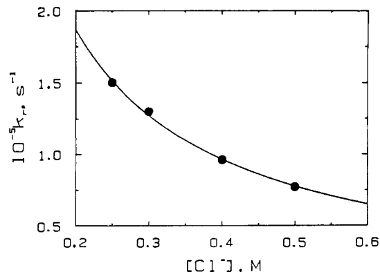
Figure 3. Rate constants from PAF measurements of the hydrolysis of \text{ICl}_2^- as a function of chloride ion concentration. Conditions: 25.0 °C, 0.50 \mu\text{M} , [\text{ICl}_2^-]_{\text{init}} = 3.0 \times 10^{-5} \text{ M} , [\text{PO}_4]_{\text{T}} = 0.6 \times 10^{-3} \text{ M} , \text{p}[\text{H}^+] = 6.50 , 230 nm.
